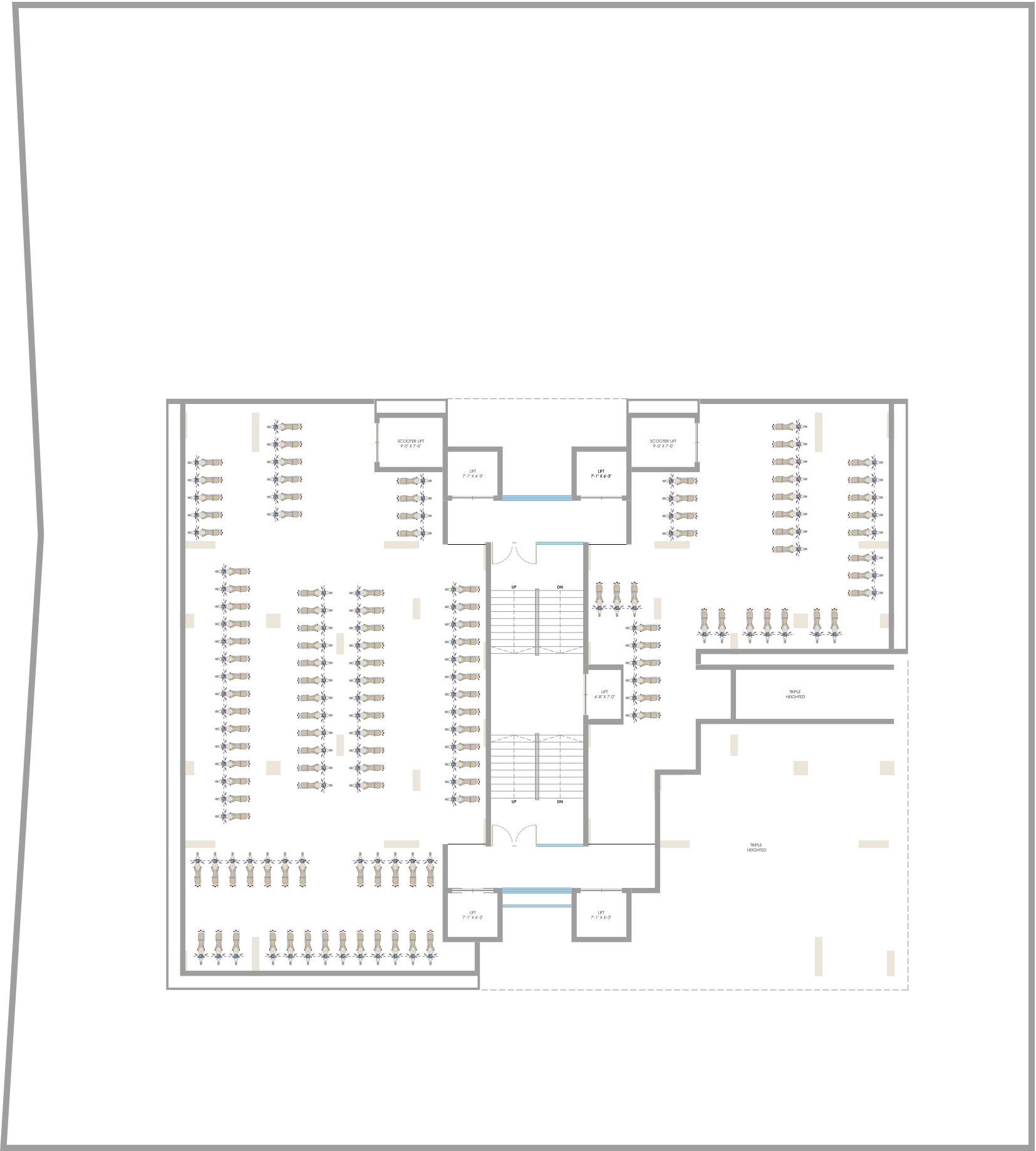
LEVEL 2 PODIUM PARKING FLOOR PLAN
